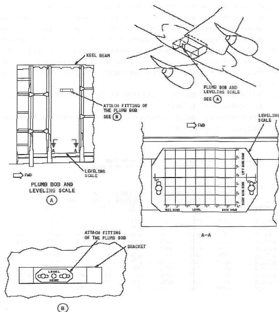
Airplane Plumb Bob and Leveling Scale
